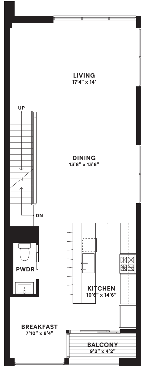
Second Floor
